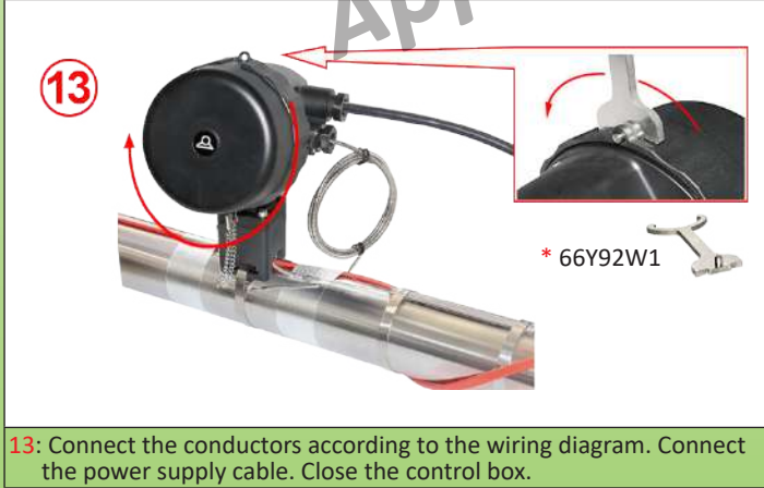
13: Connect the conductors according to the wiring diagram. Connect the power supply cable. Close the control box.
